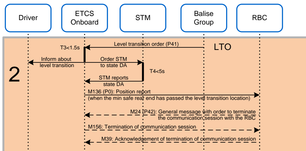
Figure 7: General sequence diagram for step 2
