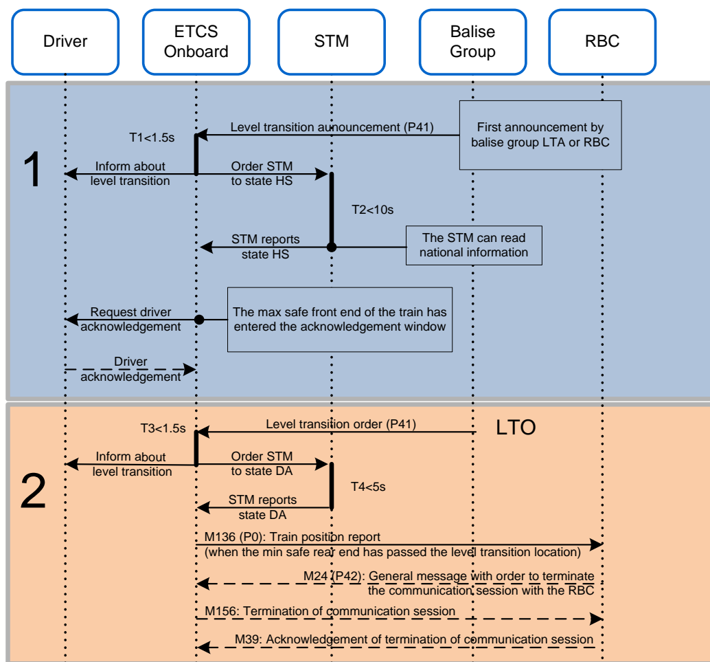
Figure 2: General sequence diagram for transition from Level 2 to level NTC
