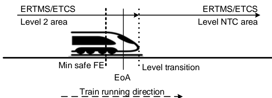
Figure 4: EOA in rear of ETCS border
