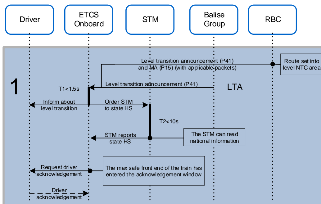
Figure 6: General sequence diagram for step 1
