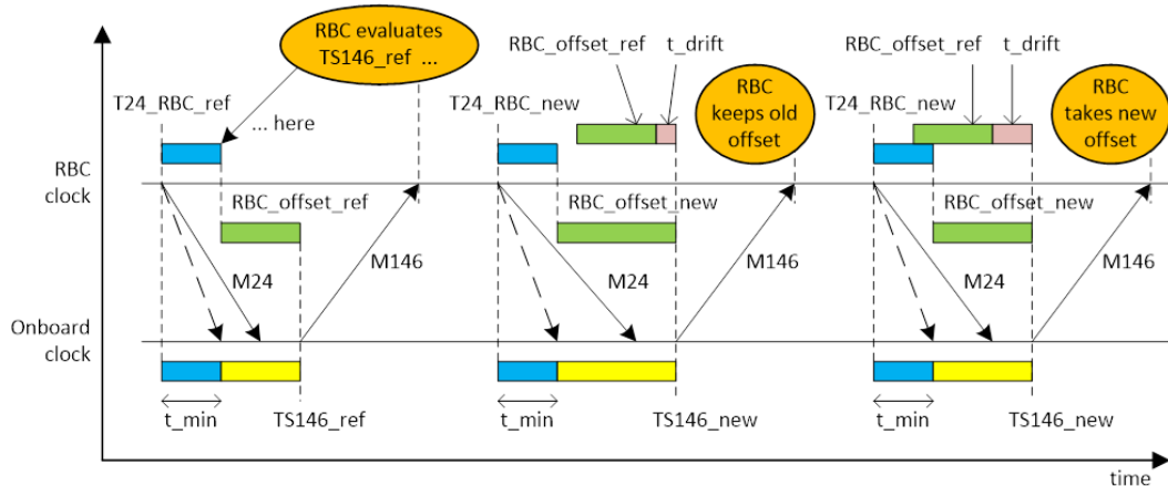
Figure 8: Clock synchronisation
