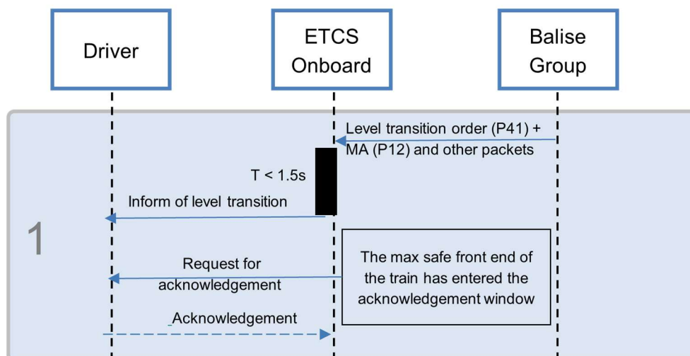
Figure 4: Sequence diagram for step 1
