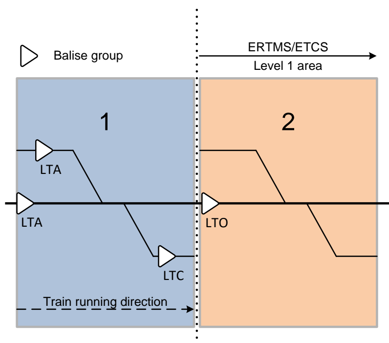
Figure 1: Generic track layout for transition from LNTC to L1
