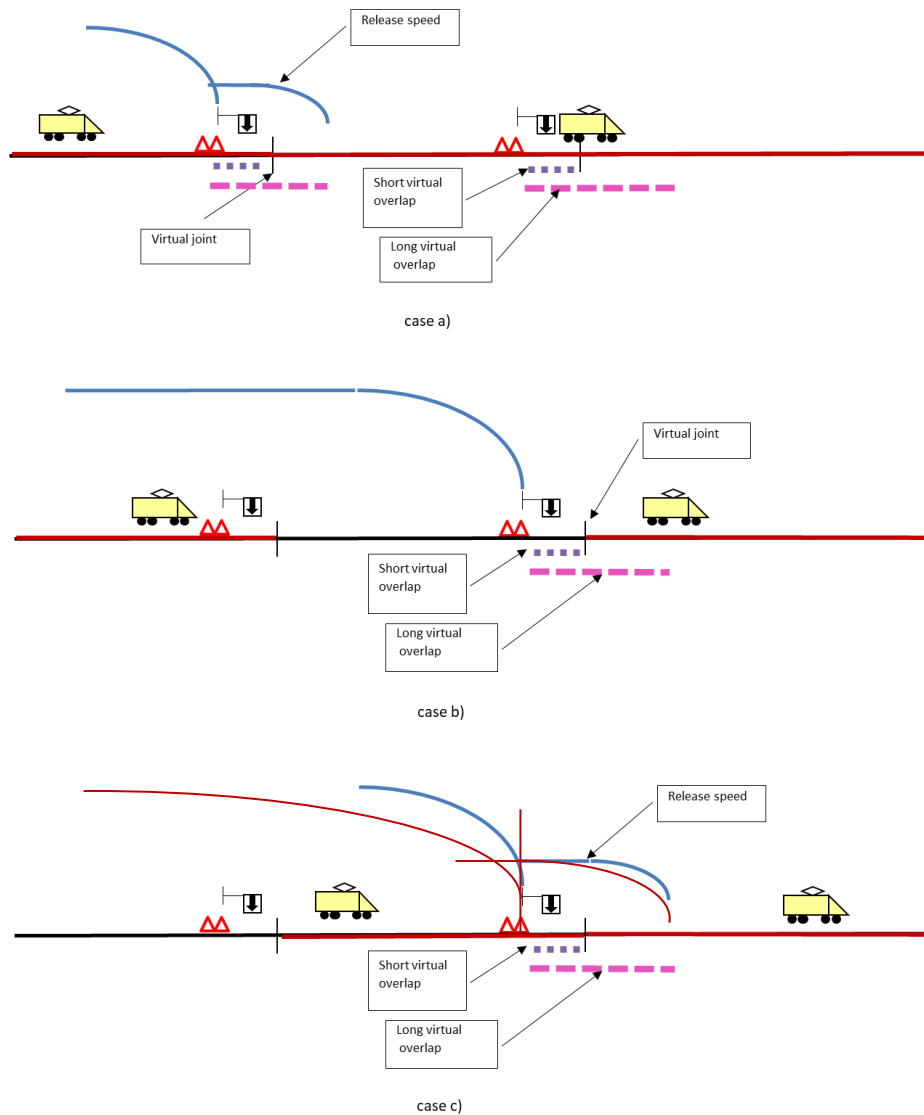
Figure 2: Case a) chased train still occupies short virtual overlap Case b) chased train still occupies long virtual overlap Case c) chased train set short and long virtual overlap free
