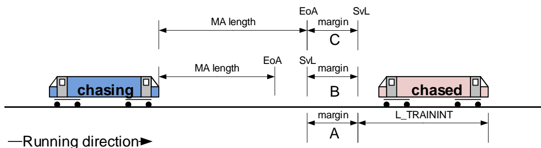
Figure 1: Margins for train position.
