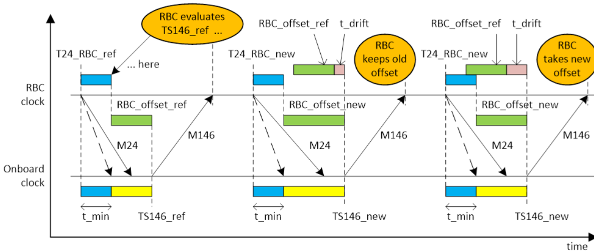
FIGURE A.1 CLOCK SYNCHRONISATION
