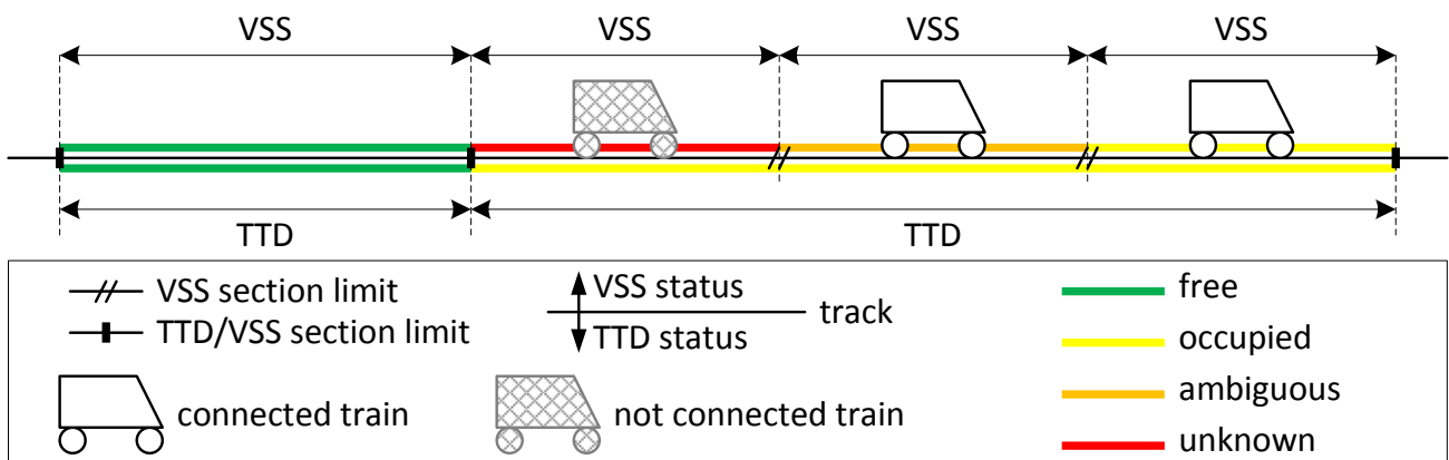
Figure 1: Section conventions
